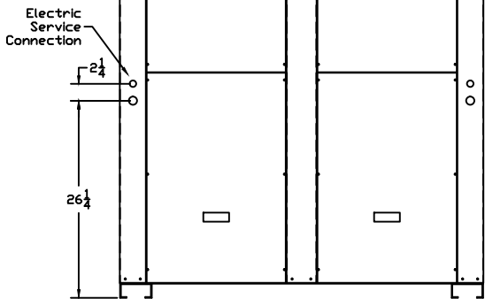
Elevation 'A'
