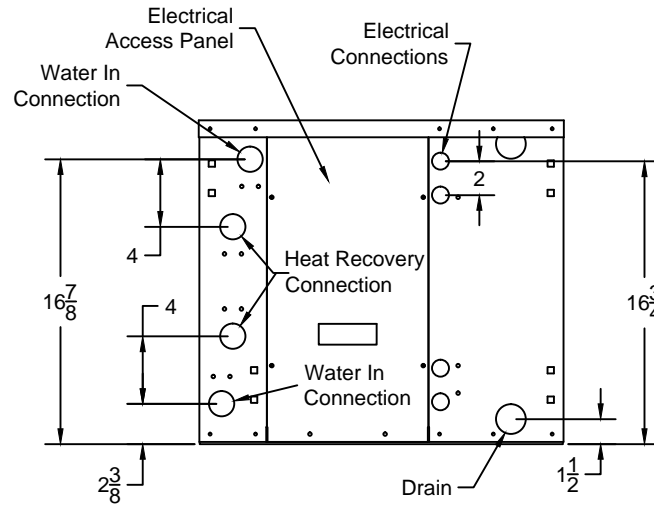
Elevation "B"
